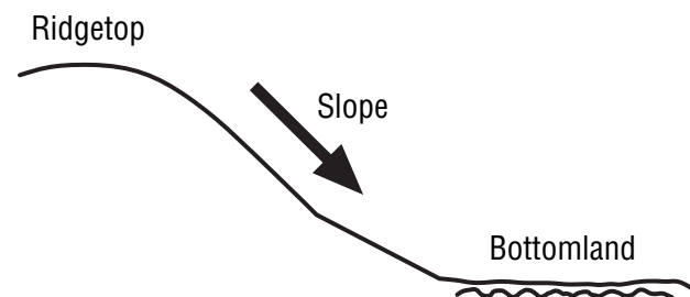
Ridgetops and slopes tend to shed water, while soils at the bottoms of slopes and in low areas collect water.
